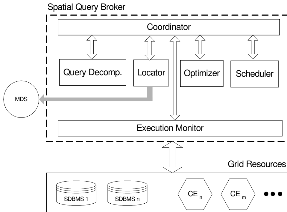
Figure 3. Spatial Query Broker architecture
