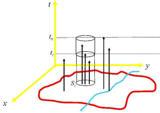
Figure 2. The estimate \hat{\mu}(C_i)
