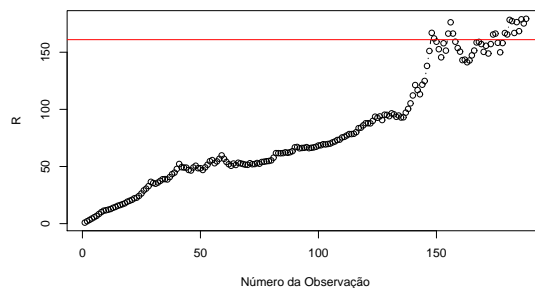
Figure 4. R_n for \varepsilon = 0.5 e \rho = 20 km
